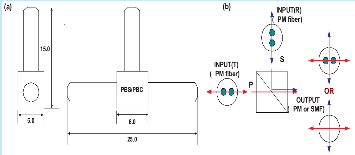
Figure 2: PBS/PBC Devices (a) Outline; (b) Polarization Orientation
