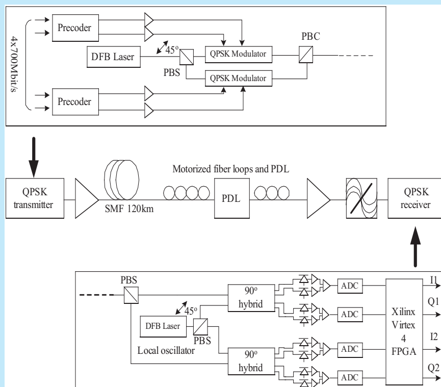
Figure 1: High Data-Rate Coherent System with PBS/PBC and PC integrated (1)
