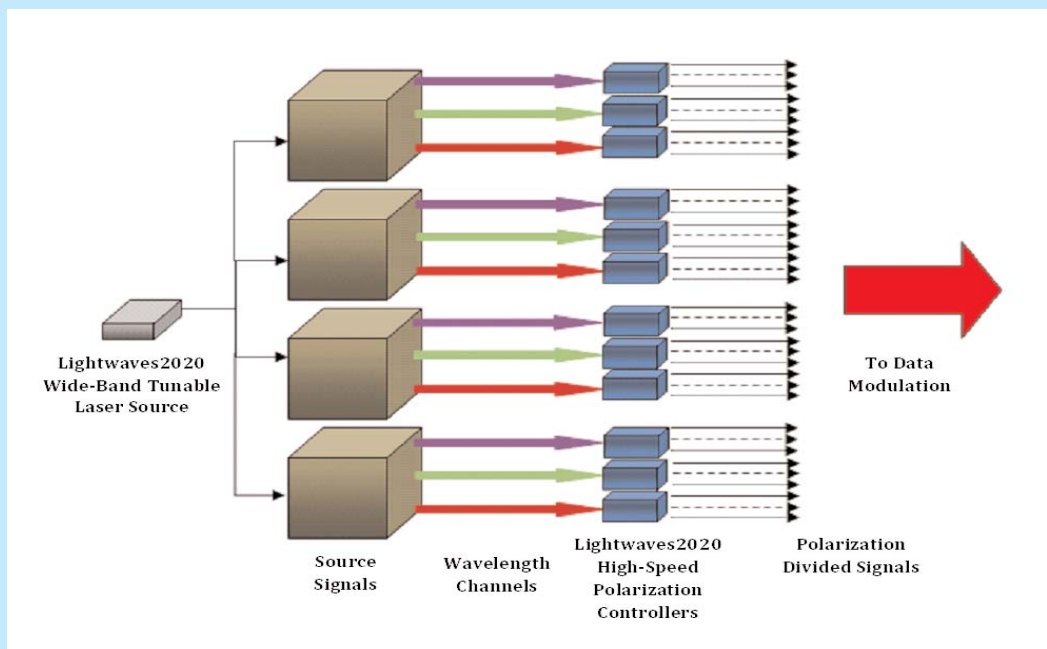
Figure 1: High Transmission Capacity with Multiple Wavelengths and Multiple Polarizations
